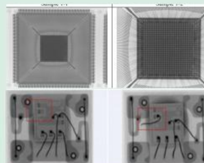
X-ray Testing
